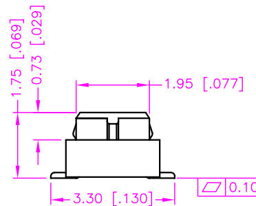
10~20PIN W/RIB
