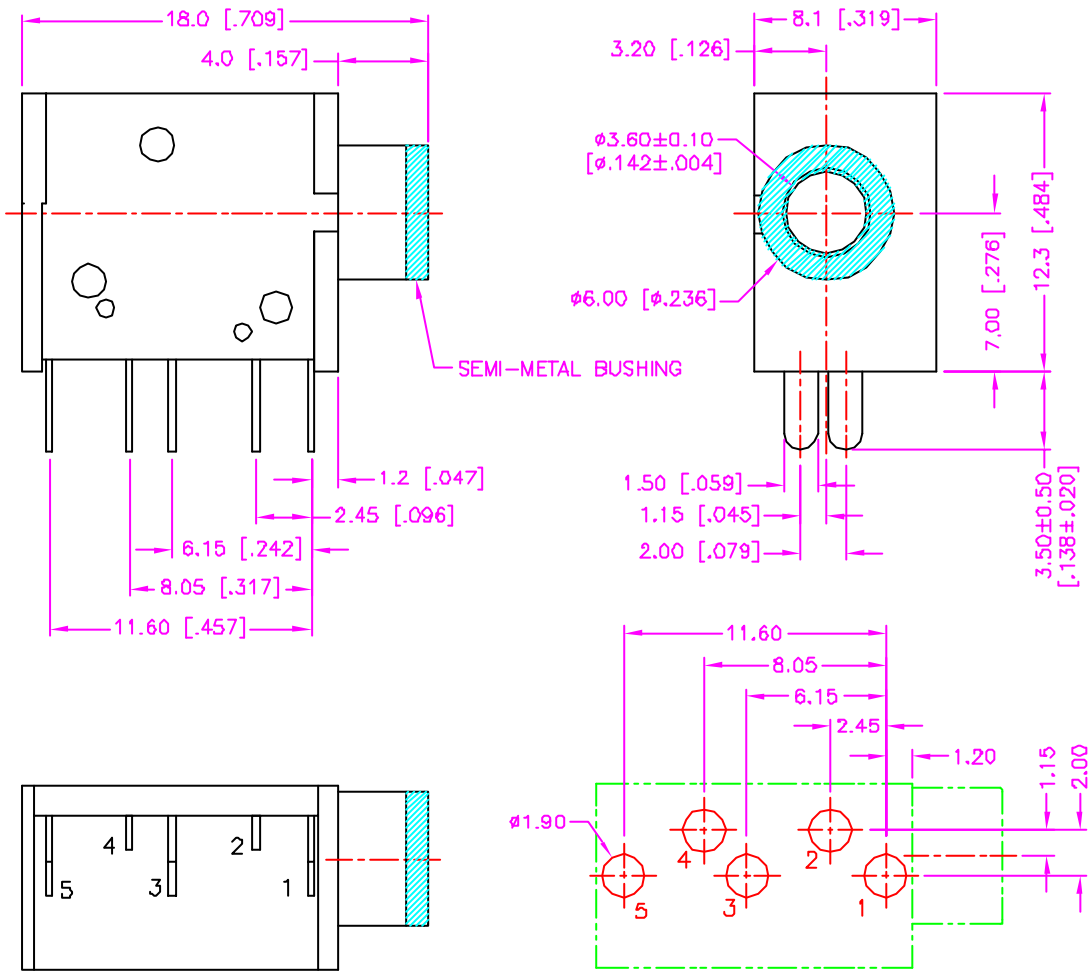
RECOMMEND P.C.B. LAYOUT BOTTOM VIEW
