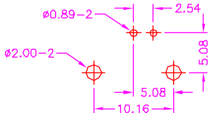
RECOMMEND P.C.B. LAYOUT TOP VIEW
