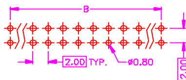
RECOMMEND P.C.B. LAYOUT BOTTOM VIEW
